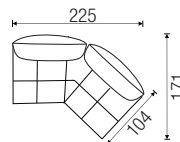
45 corner large without arm top view
