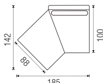
Terminal L* top view
