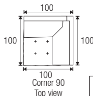
Corner 90 100x89x100
