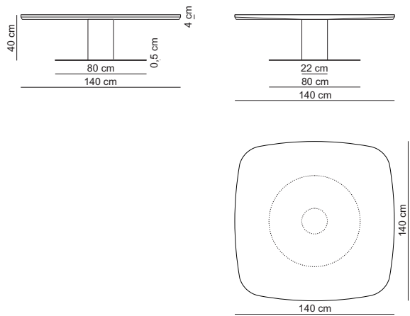
Coffee table 140x40x140 / COFTAB140
