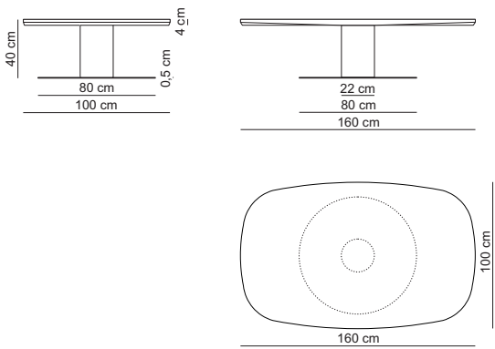
Coffee table 160x40x100 / COFTAB160X100
