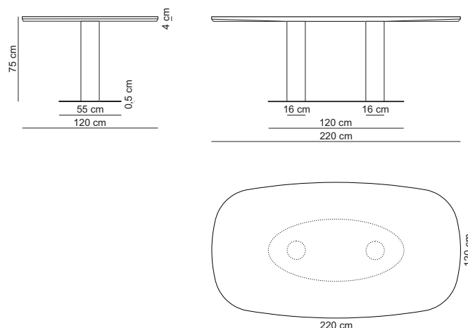
Long table 220x75x120 high / LON220X120H
