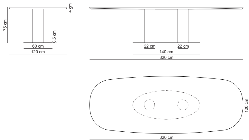
Long table 320x75x120 high / LON320X120H
