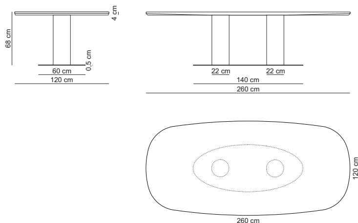
Long table 260x68x120 low / LON260X120L
