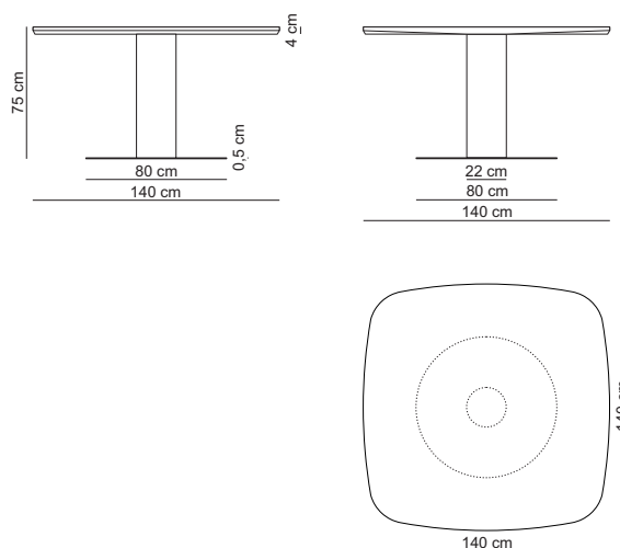
Square table 140x75x140 high / SQU140H
