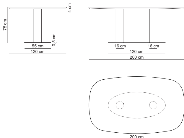
Long table 200x75x120 high / LON200X120H
