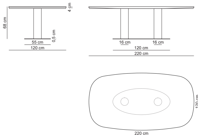
Long table 220x68x120 low / LON220X120L
