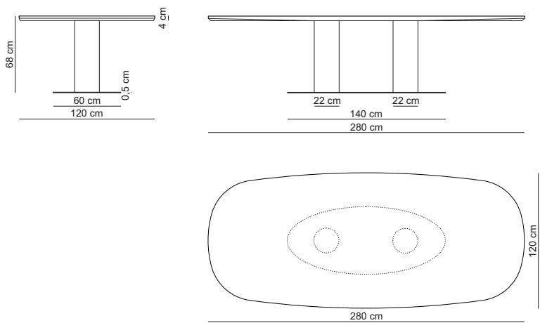
Long table 280x68x120 low / LON280X120L
