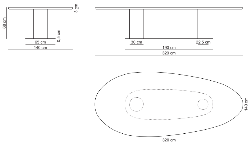
320x68x140 low / 320X140L
