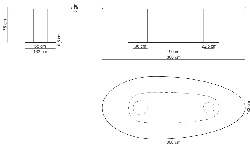
300x75x132 high / 300X132H
