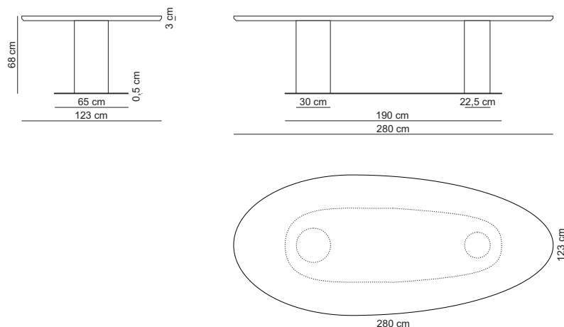
280x68x123 low / 280X123L
