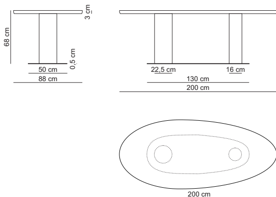
200x68x88 low / 200X88L
