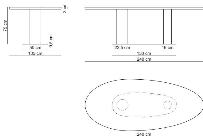
240x75x105 high / 240X105H
