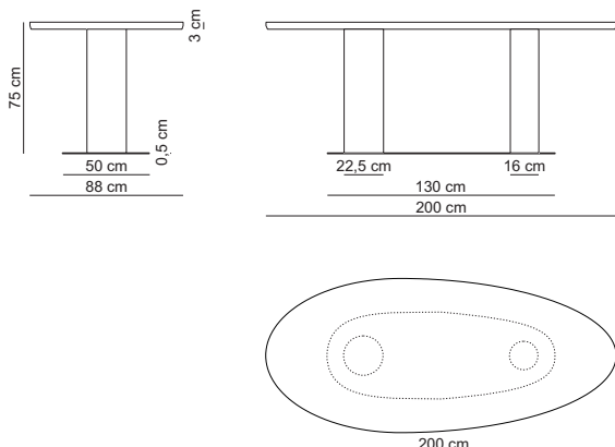
200x75x88 high / 200X88H
