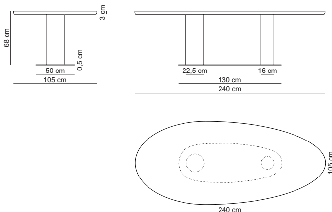
240x68x105 low / 240X105L
