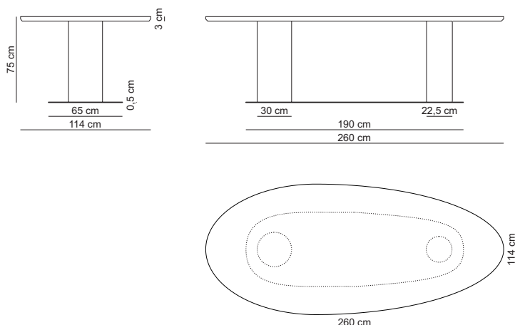
260x75x114 high / 260X114H
