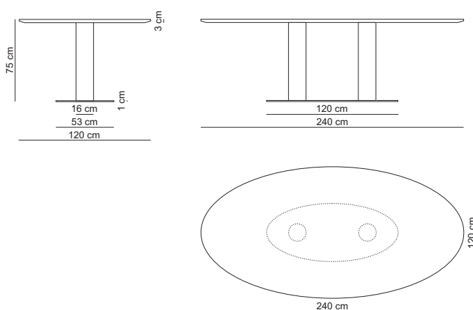
Ellipse table 240x120 high / DINLL240X120H
