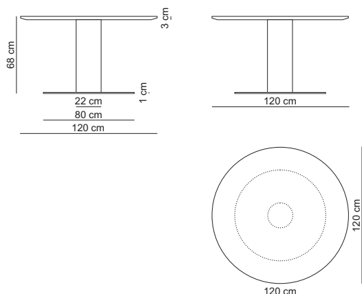
Round table 120 low / DINROU120L
