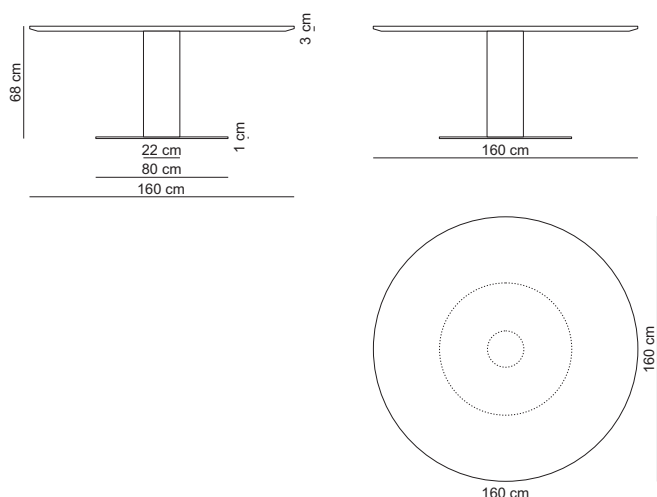
Round table 160 low / DINROU160L
