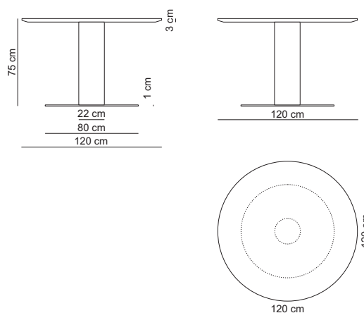
Round table 120 high / DINROU120H
