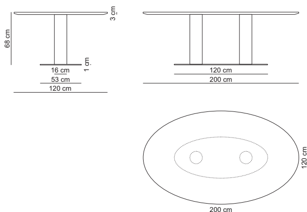
Ellipse table 200x120 low / DINLL200X120L
