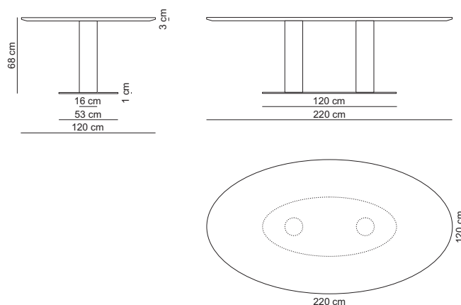
Ellipse table 220x120 low / DINLL220X120L
