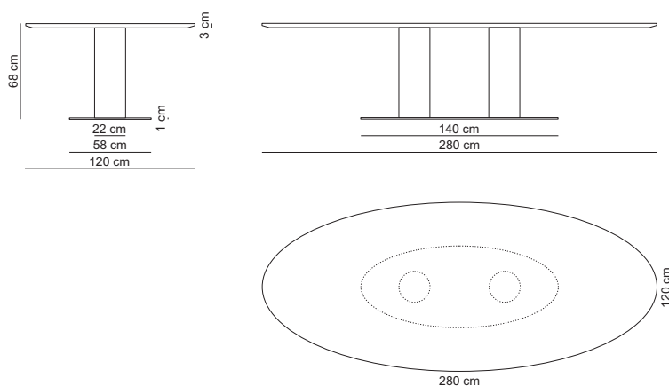
Ellipse table 280x120 low / DINCL280X120L
