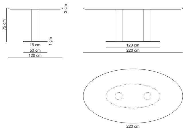
Ellipse table 220x120 high / DINLL220X120H
