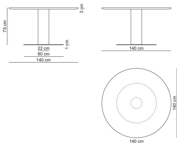
Round table 140 high / DINROU140H
