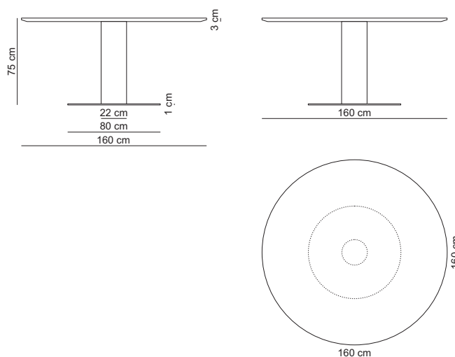
Round table 160 high / DINROU160H
