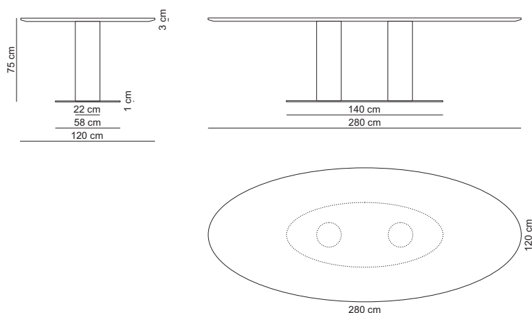
Ellipse table 280x120 high / DINCL280X120H
