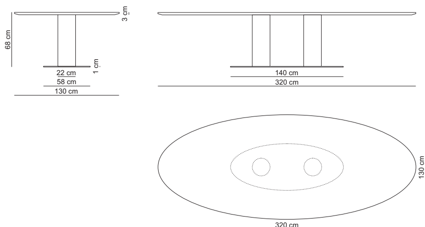
Ellipse table 320x130 low / DINCL320X130L
