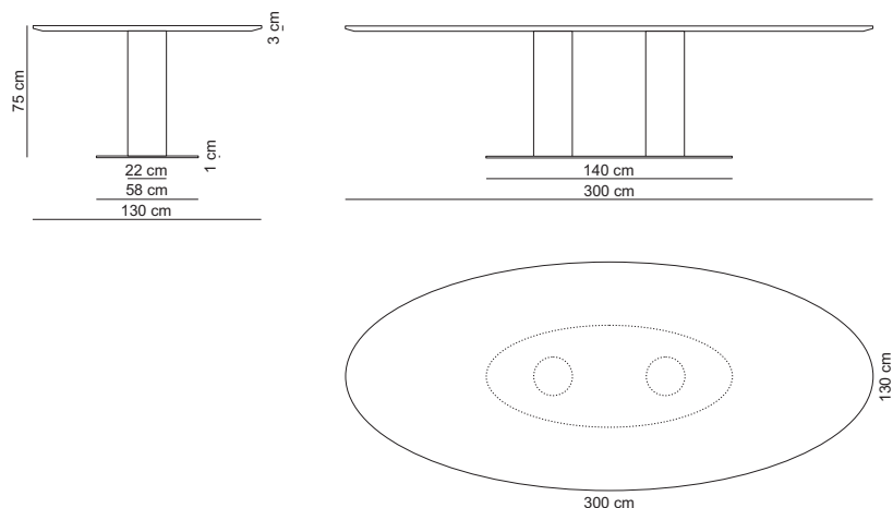
Ellipse table 300x130 high / DINCL300X130H
