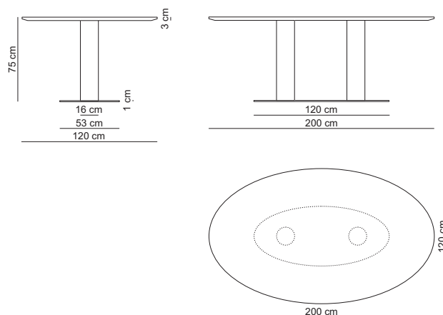
Ellipse table 200x120 high / DINLL200X120H
