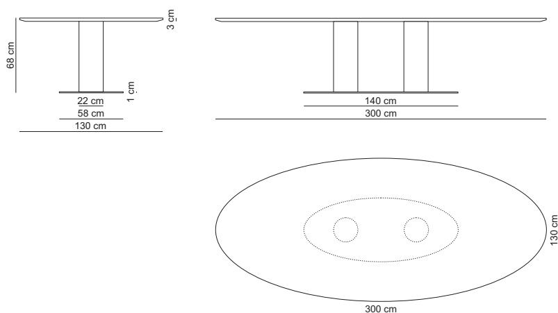
Ellipse table 300x130 low / DINCL300X130L
