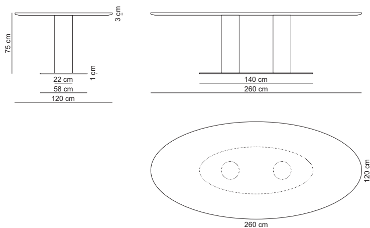
Ellipse table 260x120 high / DINCL260X120H
