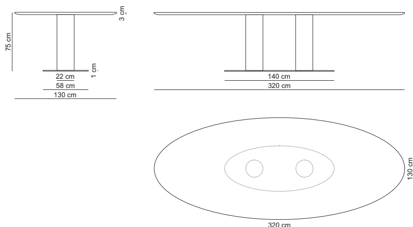
Ellipse table 320x130 high / DINCL320X130H
