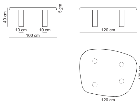
Coffee table 120 middle / TAB120M
