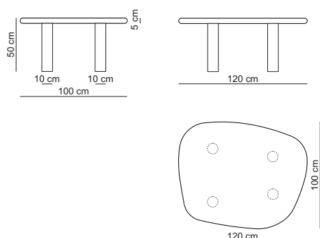
Coffee table 120 high / TAB120H
