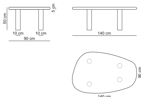
Coffee table 140 high / TAB140H
