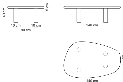
Coffee table 140 middle / TAB140M
