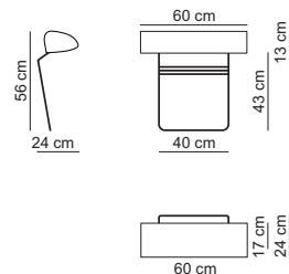
Head support / HFD15S
