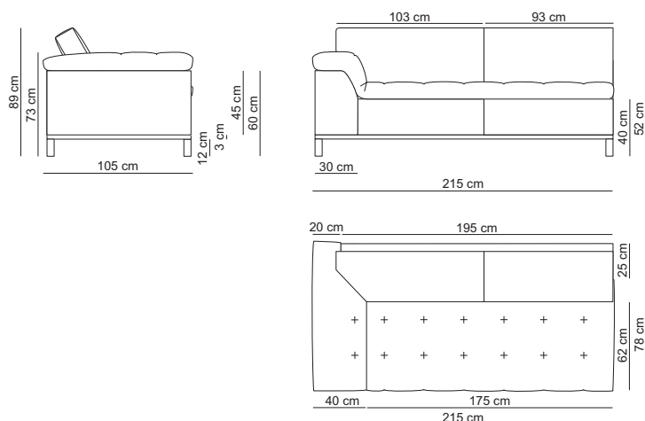
3-seat 1 arm L / 30SL
