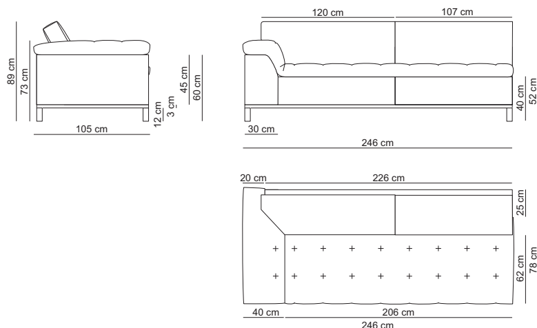
3,5-seat 1 arm L / 35SL
