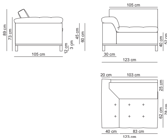
1,5-seat 1 arm L / 15SL
